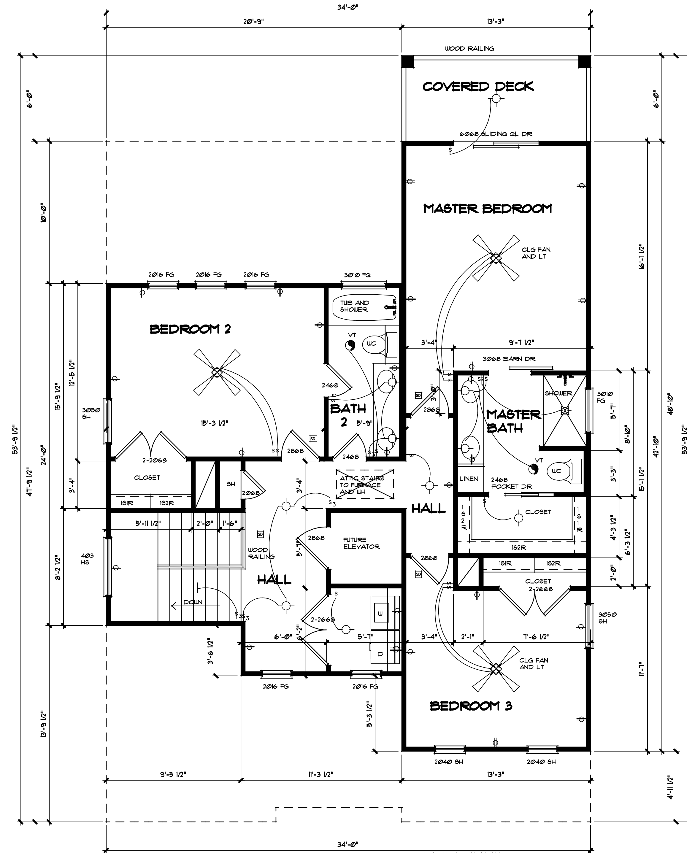
3RD FLOOR PLAN
