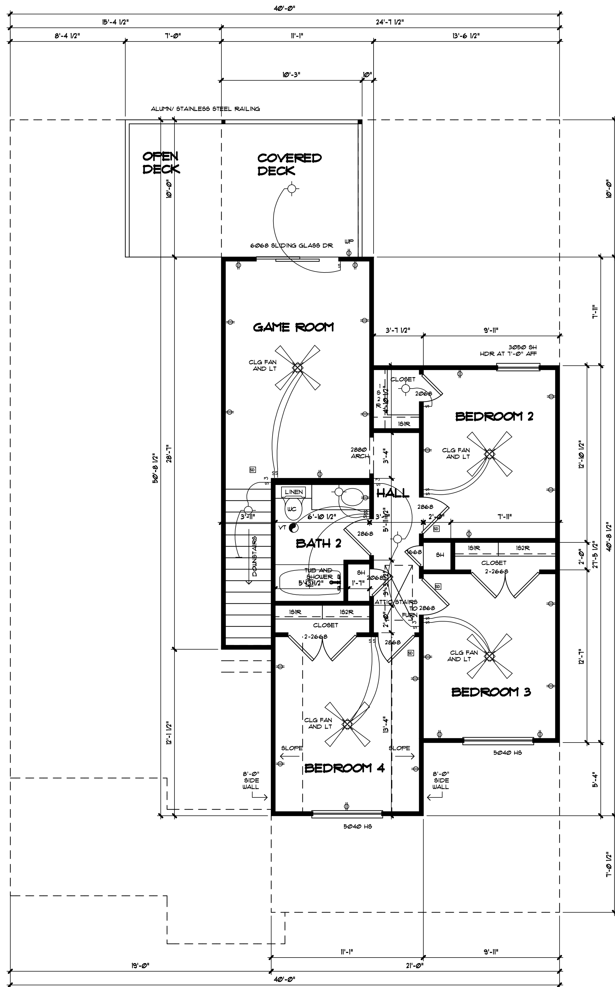
2ND FLOOR PLAN SCALE 1/4"=1'-0"
