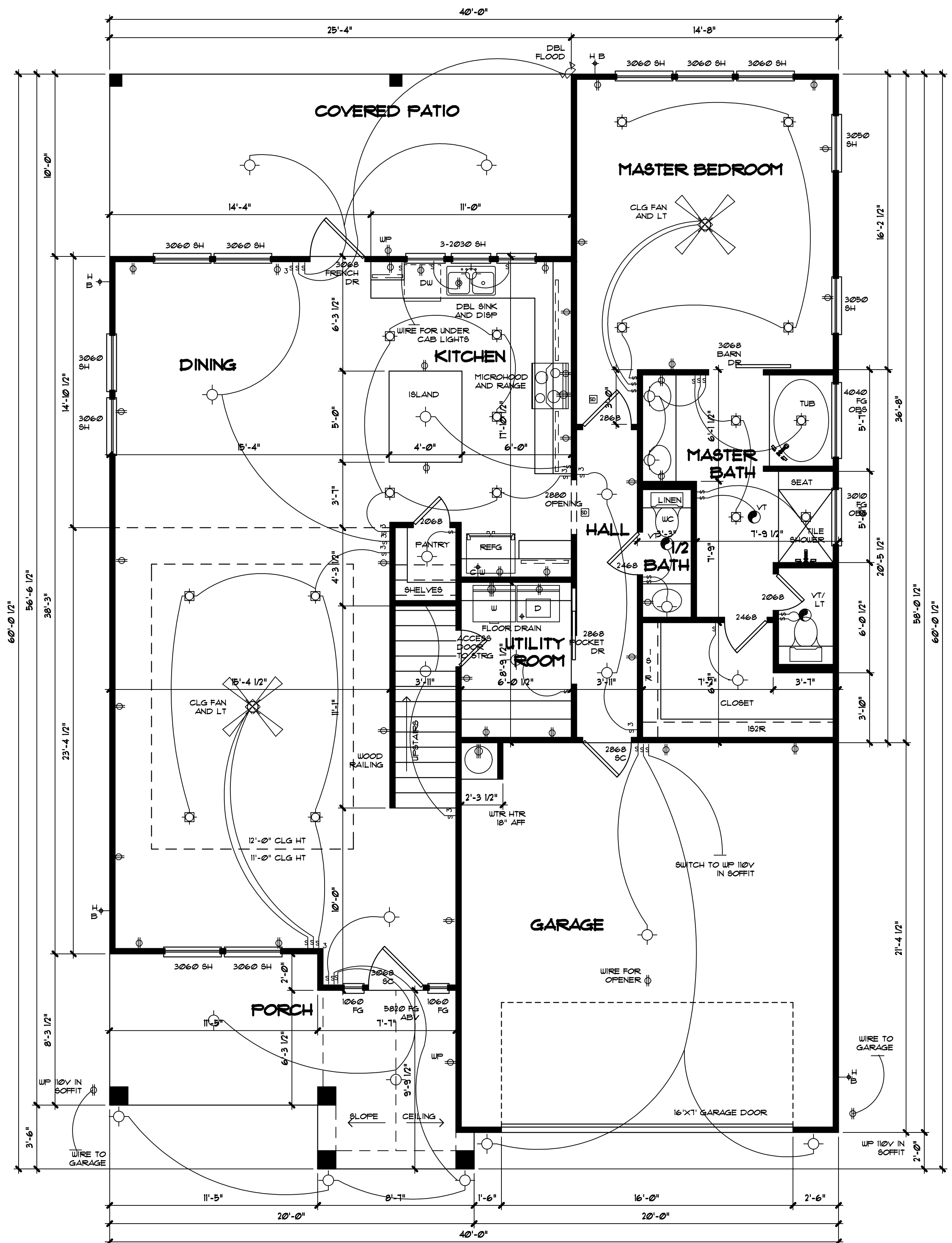
1ST FLOOR PLAN SCALE 1/4"=1'-0"
